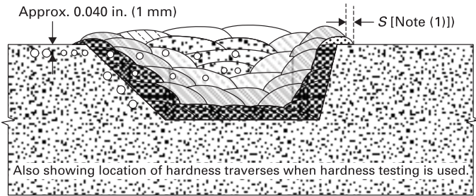
Completed Partial-Penetration Weld
