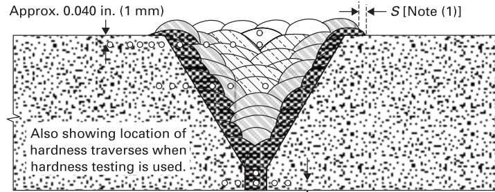
Typical Groove Weld
