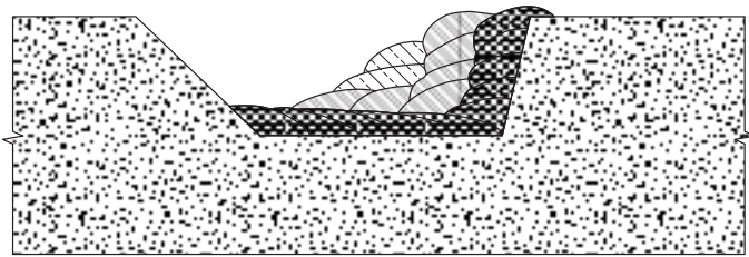
Partially Completed Partial-Penetration Weld
