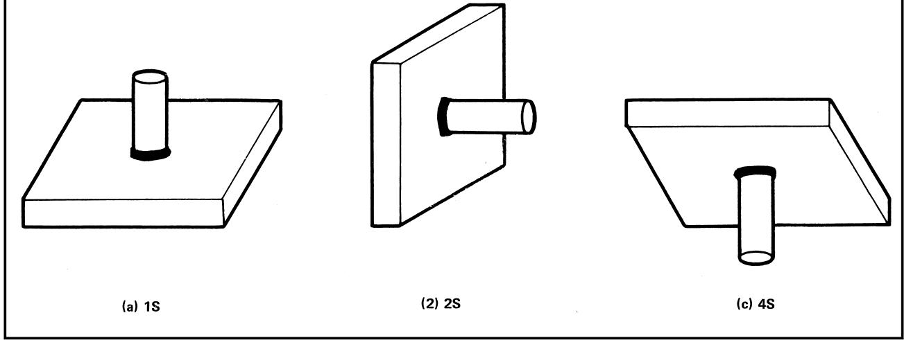
Figure QW-461.7 Stud Welds — Test Positions
