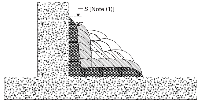
Typical Fillet Weld
